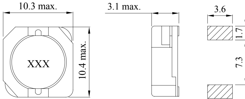
Land Pattern
